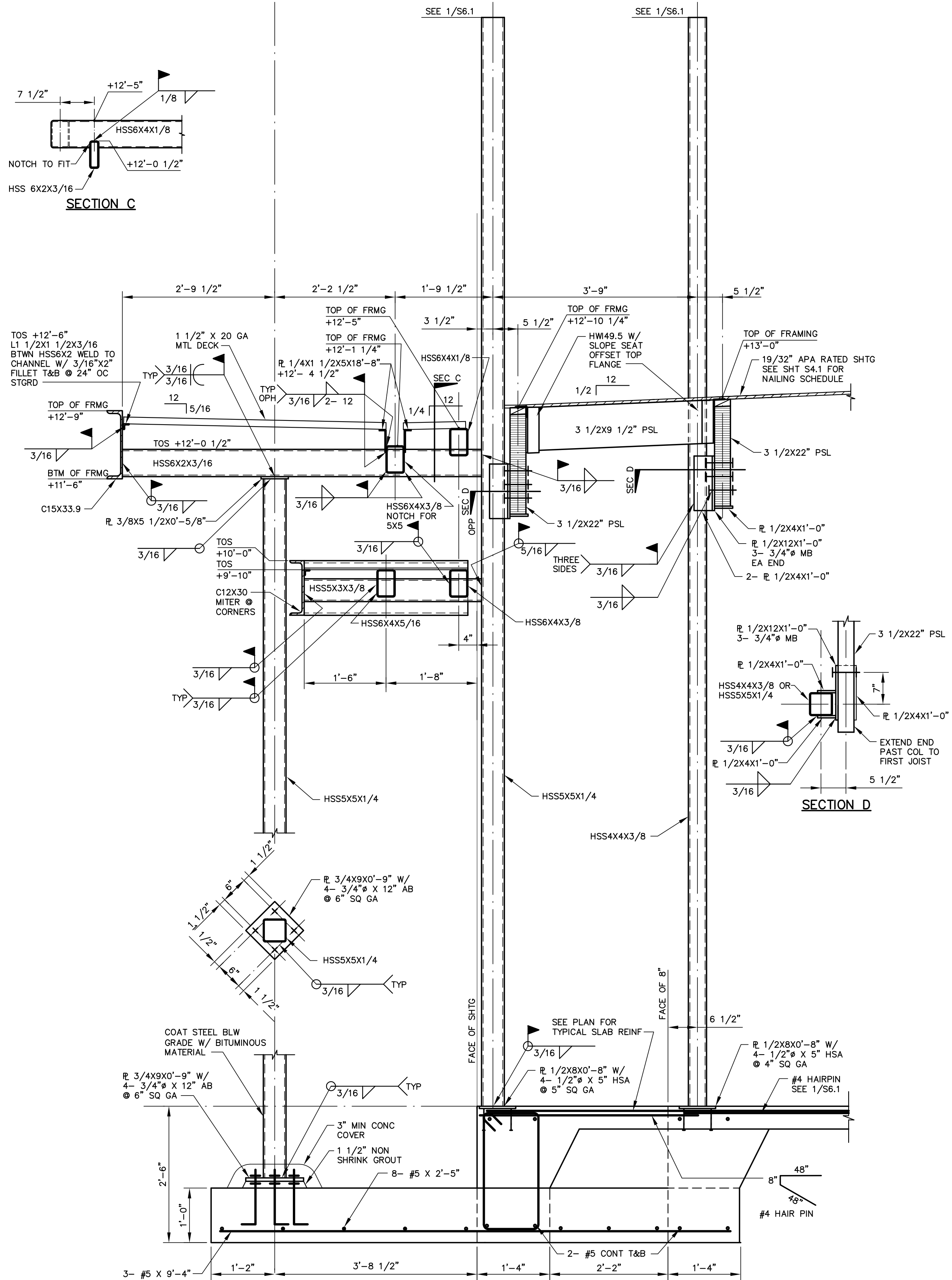
SECTION 2 S6.1 SCALE: 3/4"=1'-0"
