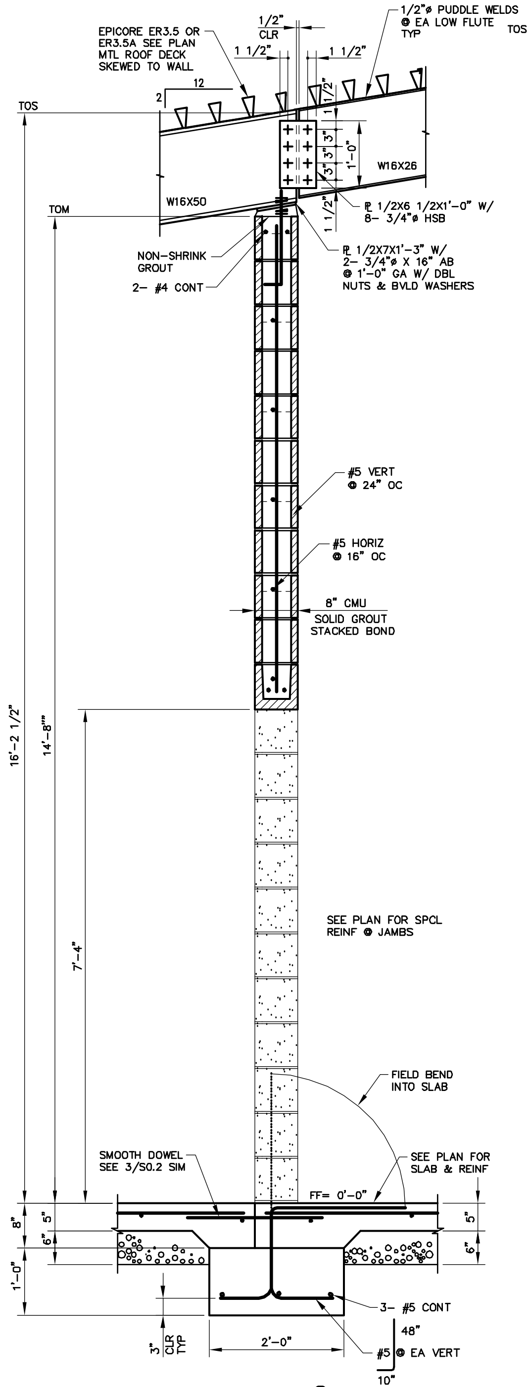
SECTION 2 AS6.4 SCALE: 3/4"=1'-0"
